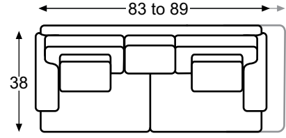
LTD7600-3C Sofa W83-89 D38 H38 W67 D22.5 H17 Seat 21 Arm 26.5
