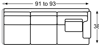
LTD7600-52 RAF Sofa W91-93 D38 H38 W80 D22.5 H17 Seat 21 Arm 26.5
