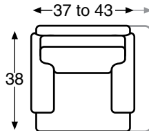
LTD7600-8 Swivel Chair W37-43 D38 H38 W21 D22.5 H17 Seat 21 Arm 26.5
