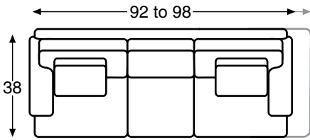
LTD7600-2 Sofa W92-98 D38 H38 W76 D22.5 H17 Seat 21 Arm 26.5
