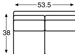
LTD7600-82 Armless Love Seat W53.5 D38 H38 W53.5 D22.5 H17 Seat 21
