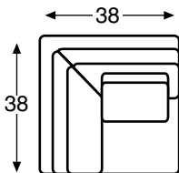
LTD7600-21 Corner Chair W38 D38 H38 W22.5 D22.5 H17 Seat 21
